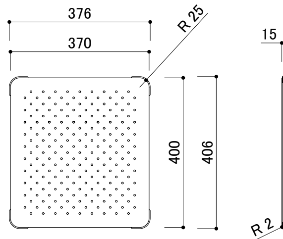
drain board (15T) 1.0T HL SUS.
