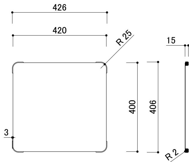
sink cover (15T) 1.0T HL SUS.
