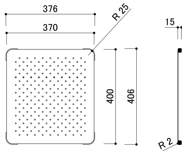
drain board (15T) 1.0T HL SUS.
